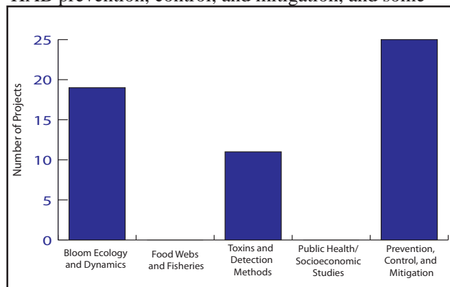
Figure 3.4. Marine HAB MERHAB projects categorized by the revised HARRNESS research categories. Projects shown include those supported beginning fiscal year 2001 through fiscal year 2008.
